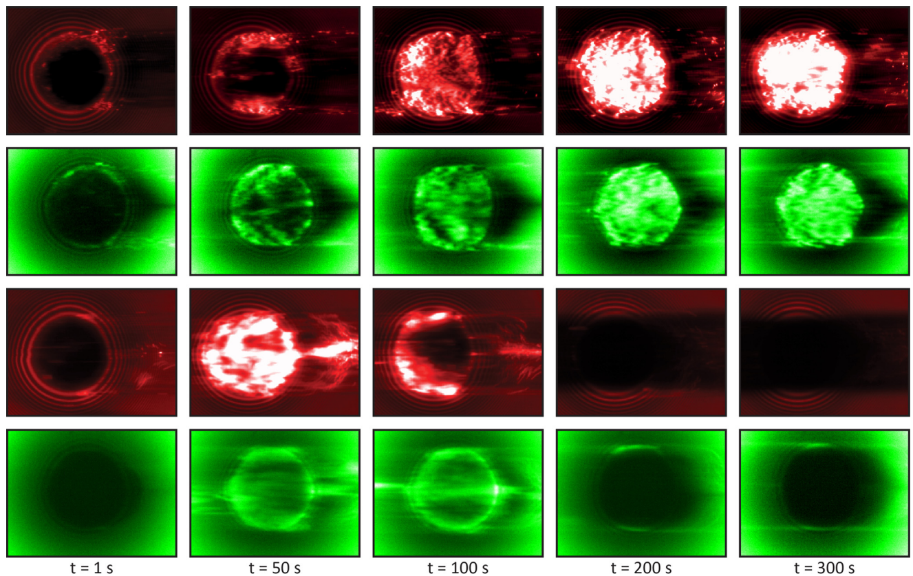
Fig. 7 – Images of the contact zone captured during the experiment under partial positive sliding (disc is faster than ball). From the top: albumin (5.7 mm/s), γ-globulin (5.7 mm/s), albumin (22 mm/s), γ-globulin (22 mm/s). The inlet is on the left of each image.
