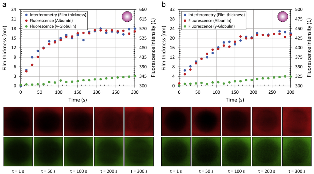
Fig. 3 – BioloX – development of film thickness and fluorescence intensity of labelled proteins as a function of time; fluorescent images of protein film in the contact zone (top – albumin, bottom – \gamma -globulin) under pure rolling conditions for different mean speeds; a) 5.7 mm/s; b) 22 mm/s.
