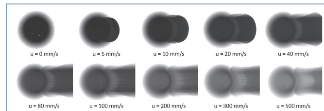
Figure 4. Film thickness maps of the lubricated compliant contact for load equal to 12 N. Inlet is on the left of each image.
