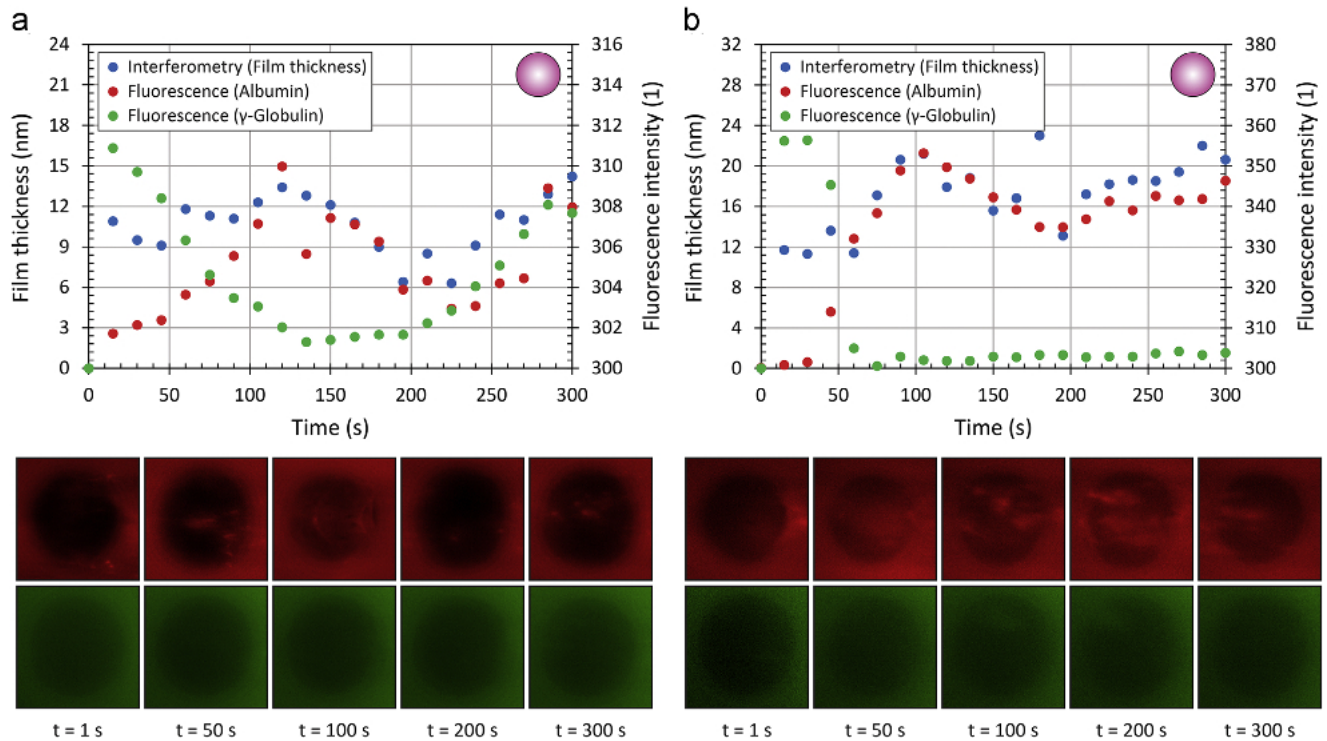
Fig. 5 – Biolog – development of film thickness and fluorescence intensity of labelled proteins as a function of time; fluorescent images of protein film in the contact zone (top – albumin, bottom – \gamma -globulin) under partial negative sliding for different mean speeds; a) 5.7 mm/s; b) 22 mm/s.
