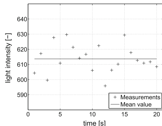
Fig. 5 Reproducibility evaluation
