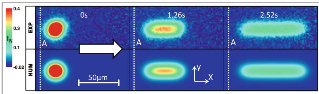
Figure 9. Validation of the methodological approach; comparison of the experimental (top) and numerical (bottom) spatiotemporal intensity distribution. White arrow indicates the shearing direction of the fluid [34].
