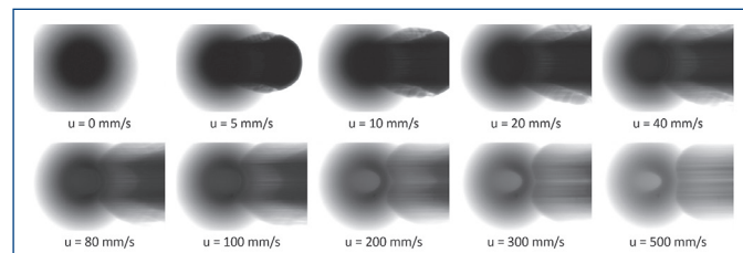
Figure 2. Film thickness maps of the lubricated PE contact. Inlet is on the left of each image.
