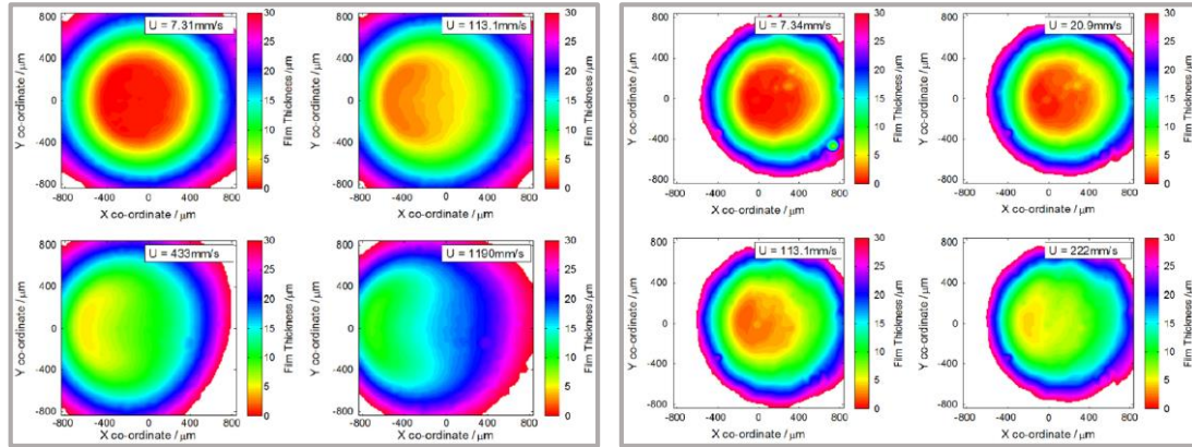
Figure 19. Film thickness maps at selected sliding speeds for PDMS pin and glass disc contact; 23.5 mN (left) and 11 mN (right) [41].
