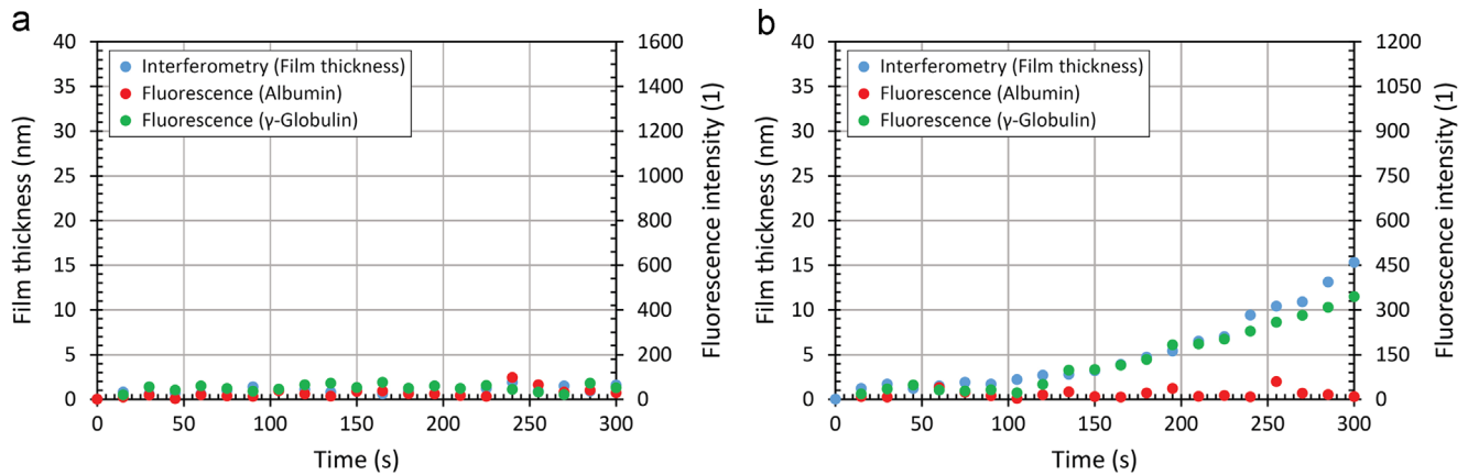
Fig. 4 – Development of film thickness and fluorescence intensity of labelled proteins as a function of time under partial negative sliding (ball is faster than disc) for different mean speeds; a) 5.7 mm/s; b) 22 mm/s.
