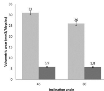
Fig 2.29 The in vitro wear rates of different inclination angle [67]
