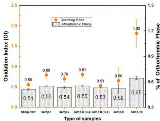
Fig. 9. Oxidation indices and percentages of orthorhombic phase for selected samples, B.A: bright area and D.A: dark area.
