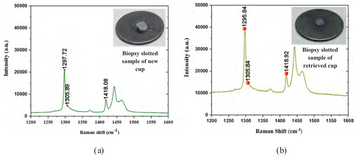
Fig. 10. Raman spectra for UHMWPE: (a) new sample and (b) sample 10. The spectra around 1305 ( I_{1305} ) represent crystallinity phase and the spectra around 1418 represent the orthorhombic phase ( I_{1418} ).
