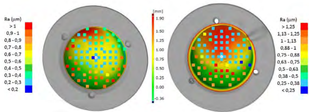
Fig 5.7 Roughness distribution on wear surface
