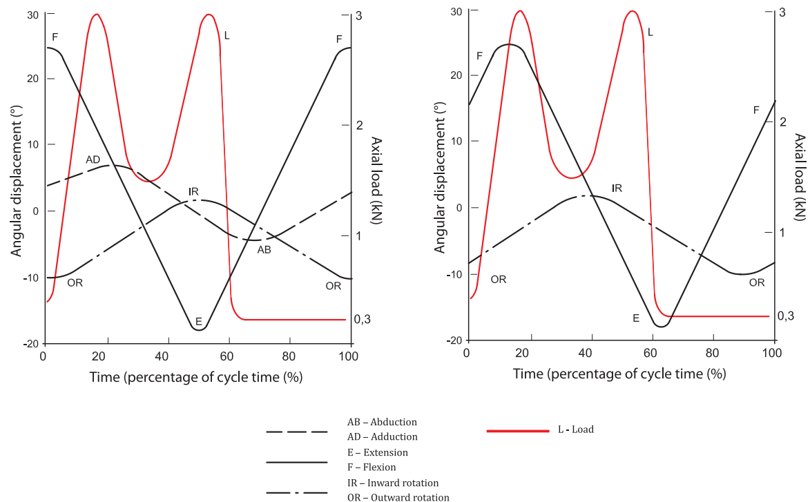
Fig. 2. Variation with time of angular movement and load to be applied to the femoral test specimen.
