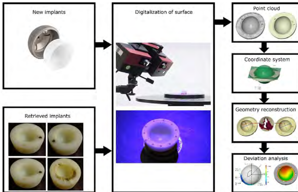
Fig 5.6 Geometry evaluation
