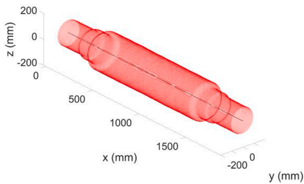
Fig. 15. Reconstructed and aligned forging geometry.
