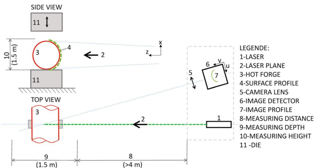
Fig. 2-33 Forging measurement using laser triangulation method [52].
