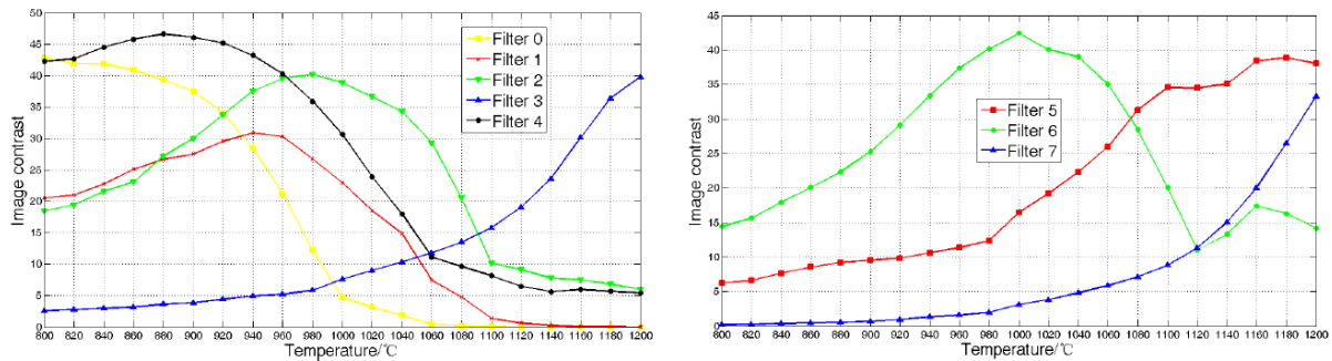
Fig. 2-5 Dependency of forging contrast on the forging temperature [14].
