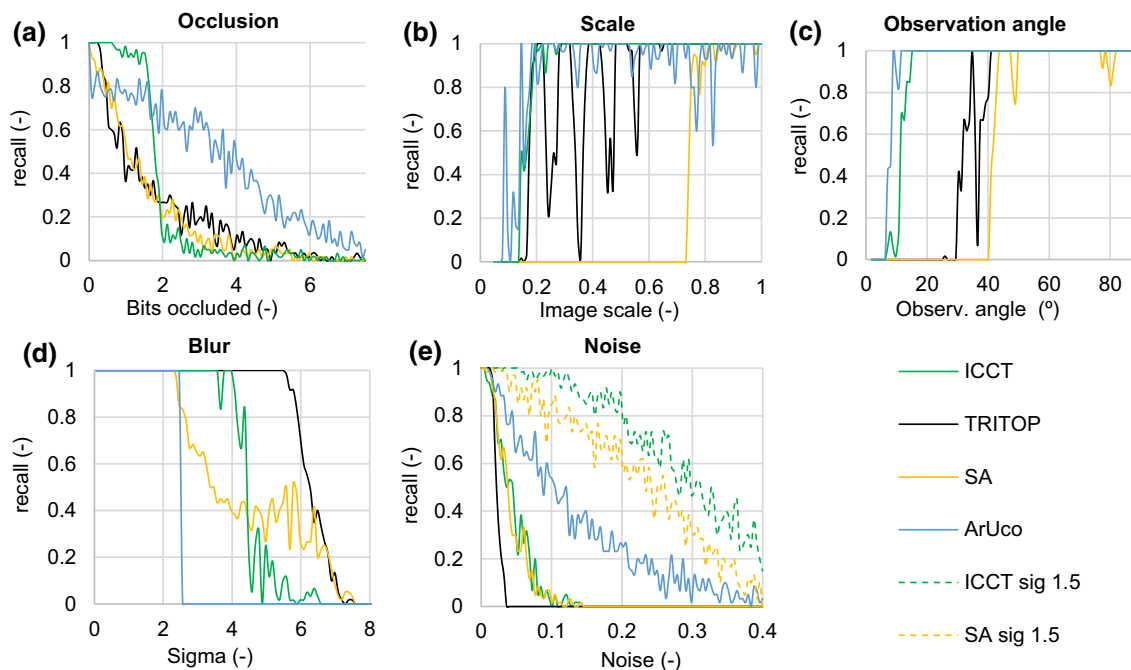
Fig. 14 Results of target recognition on synthetic datasets—a occlusion, b scale, c obs. angle, d blur, e noise (original set-up with \sigma_{\text{Canny}} = 0.5 ; set-up with \sigma_{\text{Canny}} = 1.5 )
