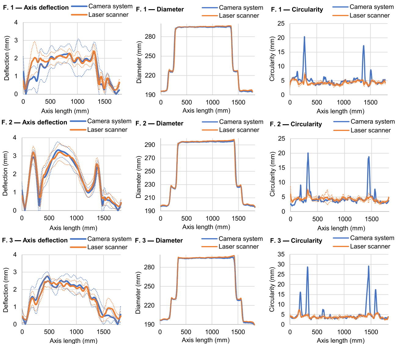
Fig. 16 Forgings 1–3 mean geometry characteristics obtained using both the camera system and laser scanner measurement methods. Dotted lines delineate the 95% confidence interval of the mean geometry
