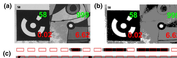
Fig. 10 Result of quantization of coded and non-coded targets. a Greyscale picture, b quantized picture, green—target’s identification number (999=unidentified), red—rotational-independent distance from the best-fit code from the code library (explained further), c—scanned and quantized codes of the targets with bit segments (red) (color figure online)
