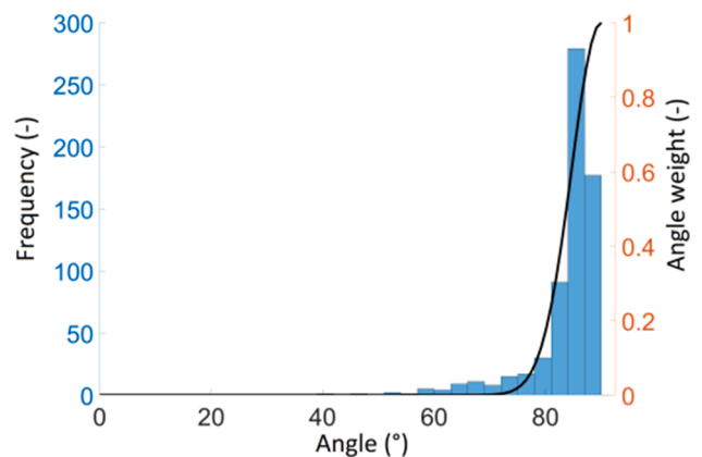
Fig. 11. Sample edge orientation histogram with its weighting function (black line) for subsequent edge filtering.
