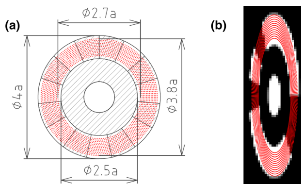
Fig. 9 Scanning for the identification code (scanning path—red points); a dimensions of the scanning area, b scanning path in the image (color figure online)
