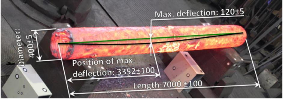
Fig. 2-49 The estimation of the accuracy of passive camera measurement system for its potential use in the industrial environment. [63].
