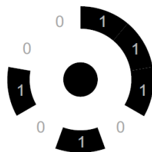
Fig. 2-18 Sample design of circular coded target often used in industrial photogrammetric applications; in the center - contrasting circle for target segmentation and location; annulus around – the unique code ring (9-bit in this case) [8].
