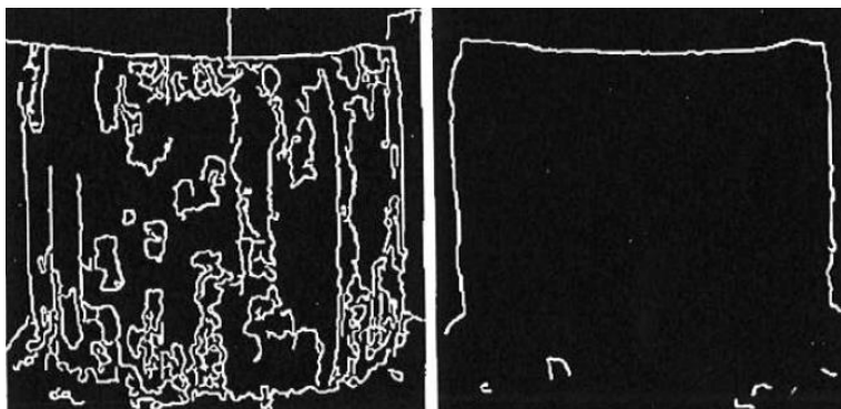
Fig. 2-6 Comparison of the forging image processed by Canny edge operator (left), and the proposed segmentation method (right) [15].
