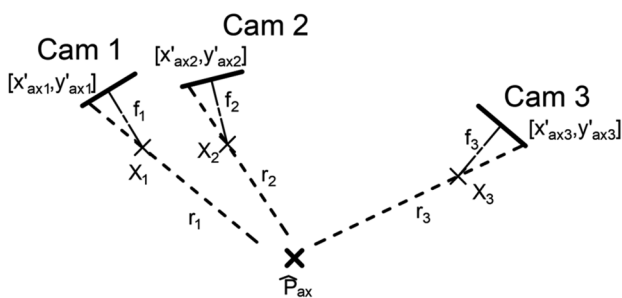
Fig. 10 Axis triangulation scheme
