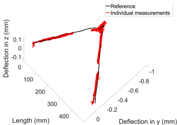
Fig. 17. Measured and reference object axis geometry.
