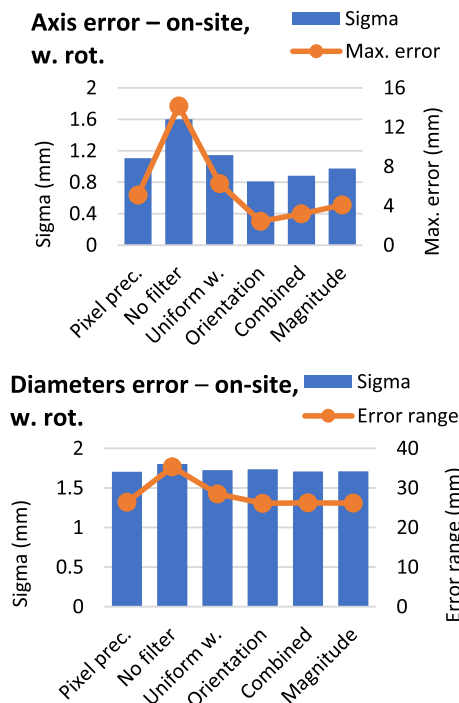
Fig. 23. Measurement method error characteristics in an industrial environment with rotation around the forging axis.
