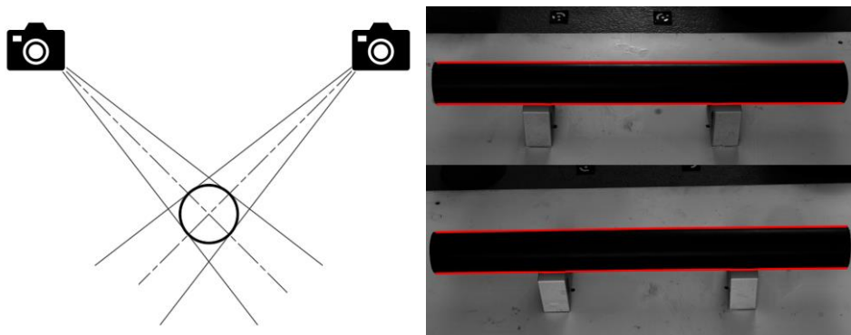
Fig. 5-1 Left - basic principle of a camera measurement system; right – example measurement images from the cameras of the system.
