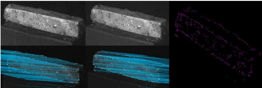
Fig. 2-38 Left – stereo images with corresponding feature points (marked blue); right – resulting 3D reconstruction of the object [56].
