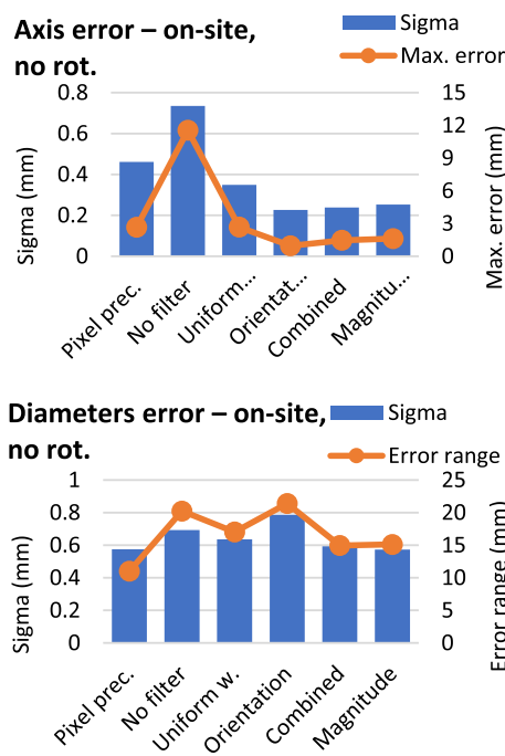
Fig. 22. Measurement method error characteristics in an industrial environment with no rotation around the forging axis.
