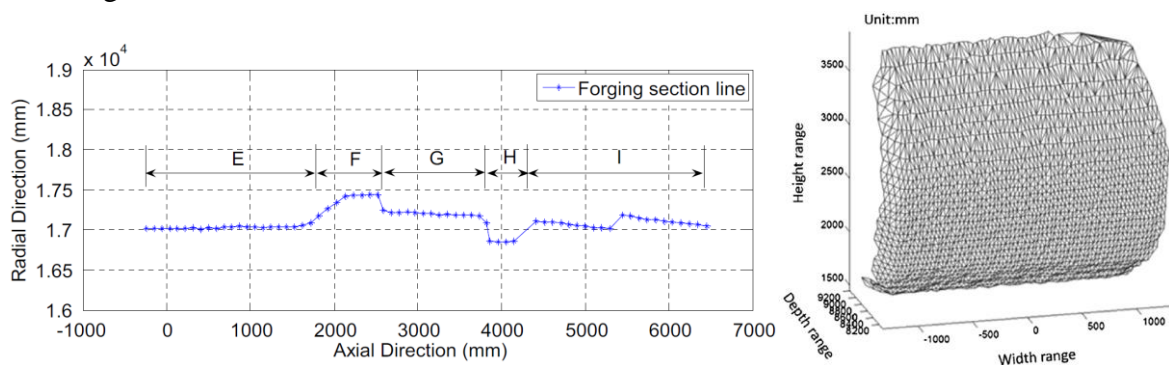
Fig. 2-22 Left – the measurement result presented by Tian [37] and Du [38].
