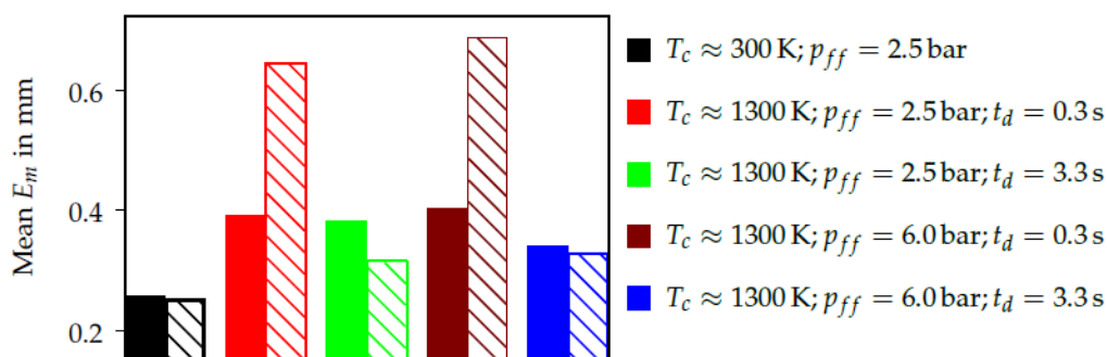
Fig. 2-14 The experimentally measured mean reconstruction error E_m in dependence on the compressed air pressure ( p_{ff} ), time from flow activation of the flow to the measurement ( t_d ). The hatched columns denote the measurement with activated air flow [21].
