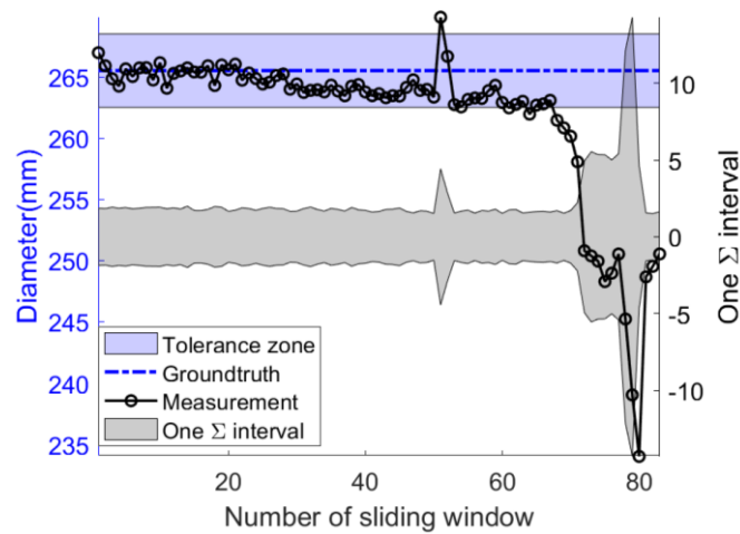
Fig. 2-43 The results of the measurement compared with the ground truth and the level of trust indicator ( \Sigma ) [60].
