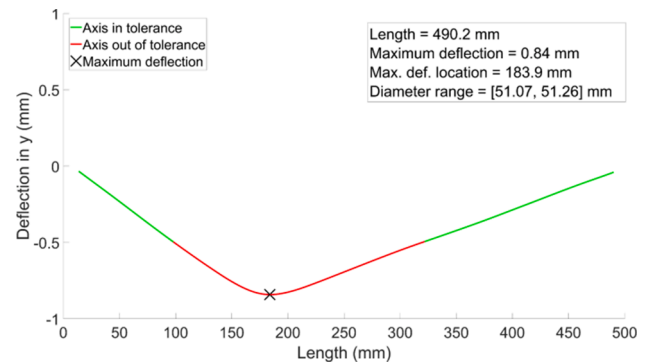
Fig. 4. Output of the forging measurement for subsequent axis straightness correction.
