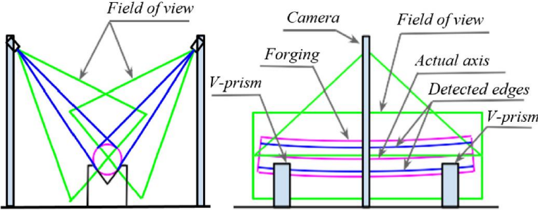
Fig. 2-44 The concept of a two-camera system for the measurement of heavy forgings [2].
