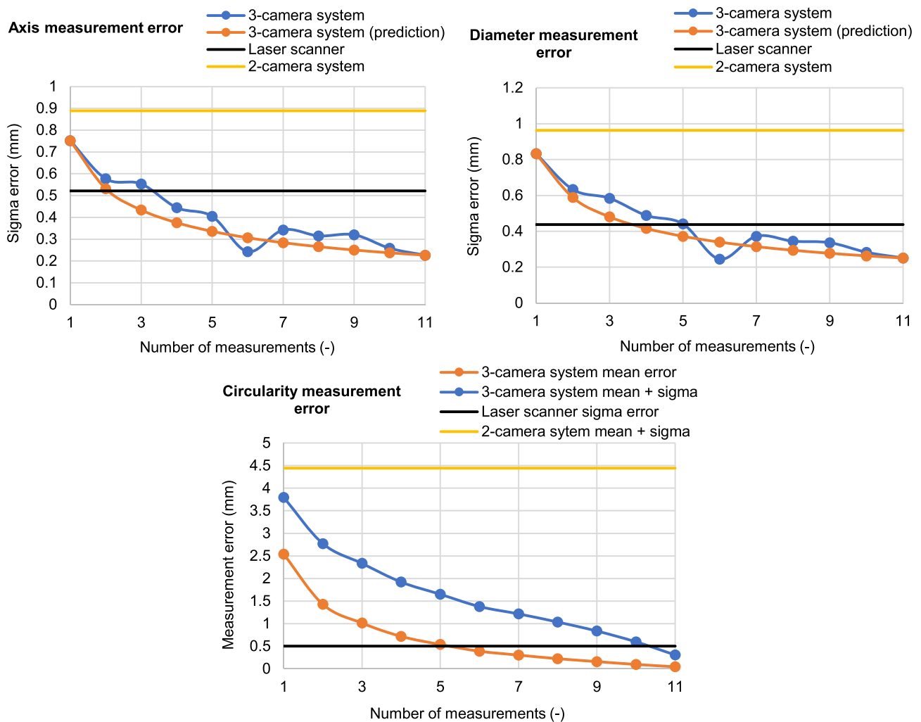
Fig. 17 Multi-observation method error compared with its prediction for the two-camera measurement and laser scanning measurement methods. Ten % of outliers were removed from the diameter and circularity results
