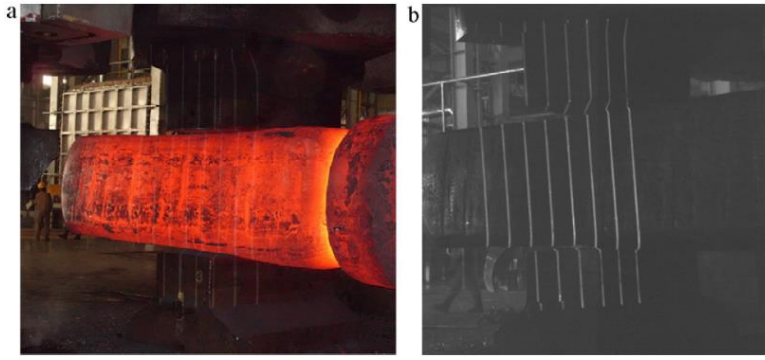
Fig. 2-8 Comparison of the measurement images without (a) and with (b) the usage of the spectral selective method [17].
