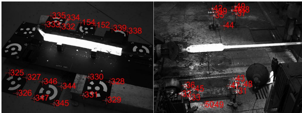
Figure 8. On the left – scene with hot forging in the laboratory, on the right – scene with hot forging in the forge, the calibration targets used for the camera calibration are marked red.
