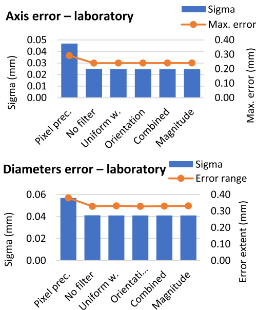
Fig. 19. Measurement error characteristics in the laboratory environment.
