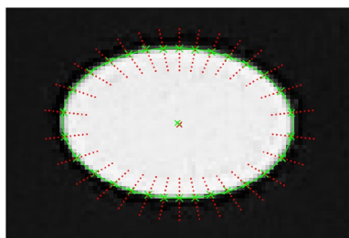
Fig. 8 Example of star ellipse operator. Red cross—initial point, red points—scanning points, green crosses on the boundary—edge points, green line—fitted ellipse, green cross in the centre—centre of the fitted ellipse (color figure online)
