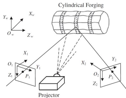
Fig. 2-24 Structured light aided stereo vision forging measurement system; camera parameters O , X , Y , Z are known, P_1 and P_2 are the corresponding image points of an object point [42].
