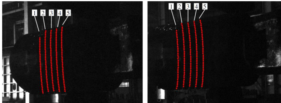
Fig. 2-26 The stereo images from the measurement system with triangulated points on the fringes 1 – 5 (marked red) [42].
