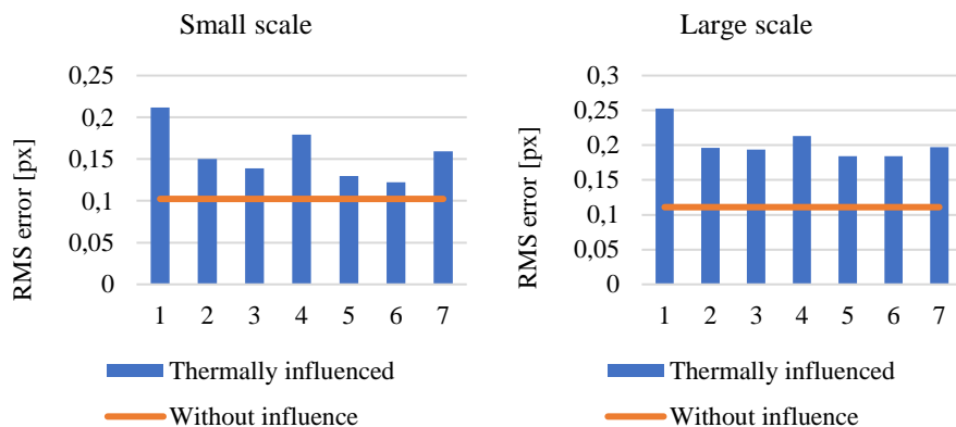
Figure 9. RMS reprojection errors of extrinsic camera parameters from particular images.
