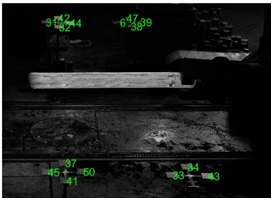
Fig. 16 Image with calibration targets from optical measurement system for the quality control of heavy forgings
