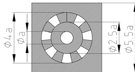
Fig. 3 Geometry of coded target, 15-bit code—0101010101010
