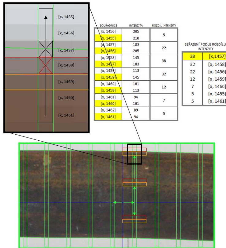
Fig. 2-46 Detection of the edge points, based on image gradient. A section of the original image with magnified edge; yellow and red windows are used to search for approximate edge; black window in the magnified image is used to search for the gradients around the edge; the table in center shows the pixel coordinates, their intensities and the difference of the intensities of neighboring pixels; the table on the right shows the intensity values from the highest to the lowest, with their coordinates, and the selected edge point marked yellow [63].
