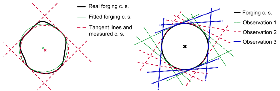
Fig. 4 Left: single-observation measurement of irregular forging cross-section and error of the measured cross-section with respect to fitted cross-section. Right: multi-camera, multi-observation measurement
