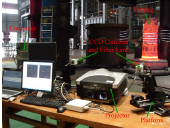
Fig. 2-7 Structured light aided stereo vision experimental setup [17].
