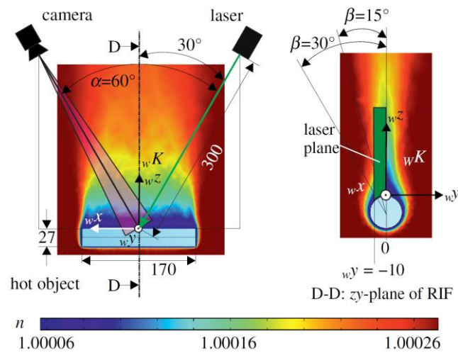
Fig. 2-11 Air lens simulation layout ( n is a local refractive index of air) [20].
