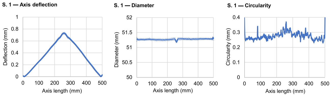
Fig. 18 Specimen 1 mean geometry characteristics measured in the laboratory environment. Dotted lines delineate the 95% confidence interval of the mean geometry
