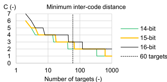
Fig. 5 Achieved minimum inter-code distance for target sets
