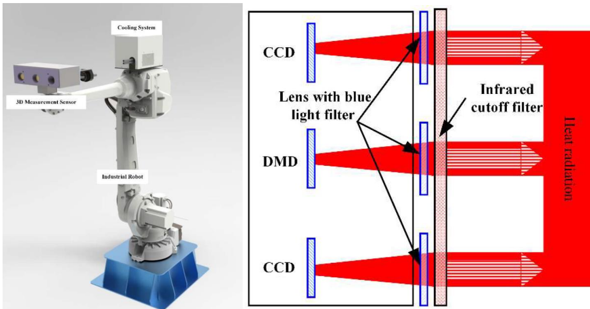
Fig. 2-29 Left - robot-driven fringe projection measurement system, right – sensor setup with a projector, 2 CCD cameras and dual optical filter [48].
