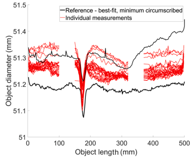
Fig. 18. Measured and reference object diameters.
