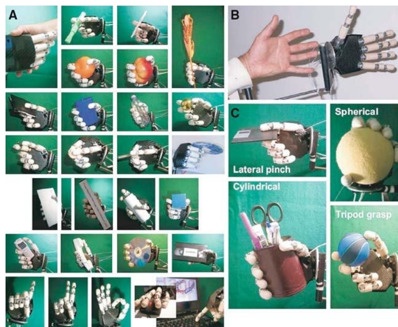
Obr. 37 CyberHand [47]
